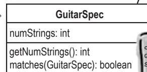
GuitarSpec.java
