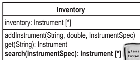
Inventory.java
